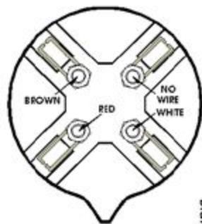
WIRING - TRAILER PLUG VIEWED FROM CABLE END
