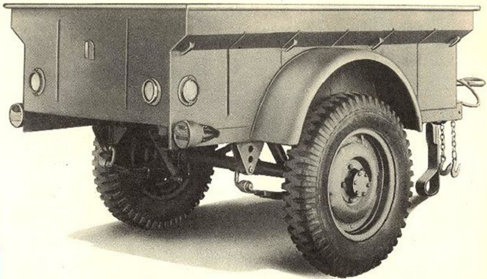
FIGURE A—TRAILER, 1/4-TON PAYLOAD, 2-WHEEL, CARGO, 1942-43, AMERICAN BANTAM T-3 AND WILLYS MBT THREE QUARTER RIGHT REAR VIEW
