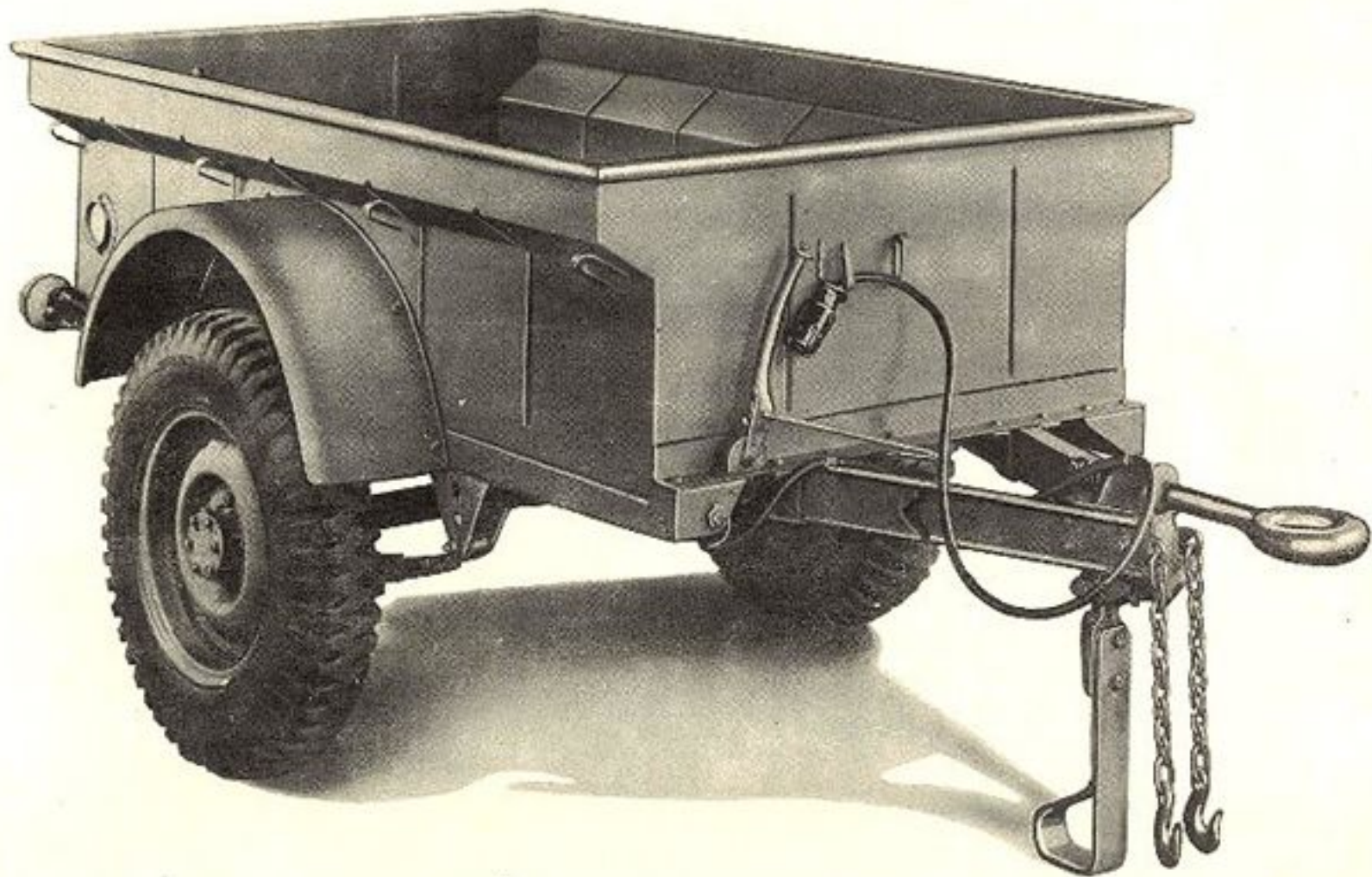
FIGURE B—TRAILER, ¼-TON PAYLOAD, 2-WHEEL, CARGO, 1942-43, AMERICAN BANTAM T-3 AND WILLYS MBT THREE QUARTER RIGHT FRONT VIEW
